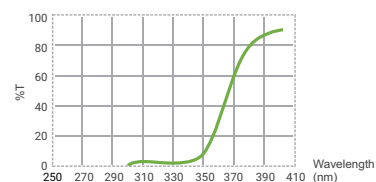
SPECTRAL TRANSMITTANCE
