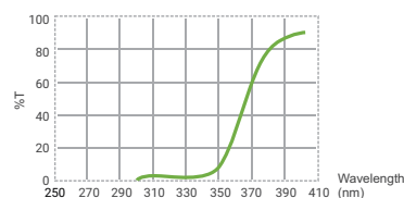
SPECTRAL TRANSMITTANCE
